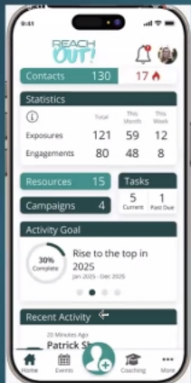
Dashboard
